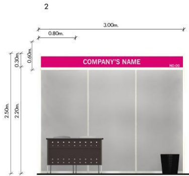
FRONT VIEW SCALE 1:50
