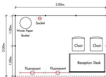
LAYOUTPLAN SCALE 1:50
